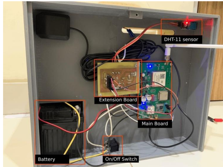
Fig. 8. SmartBox Device Front Look
