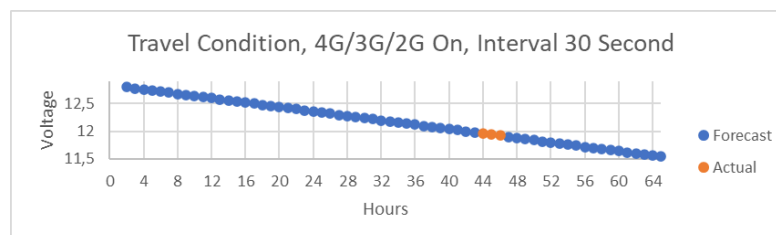
Fig. 7. Battery Life Test When Sending Data Every 30 Seconds
