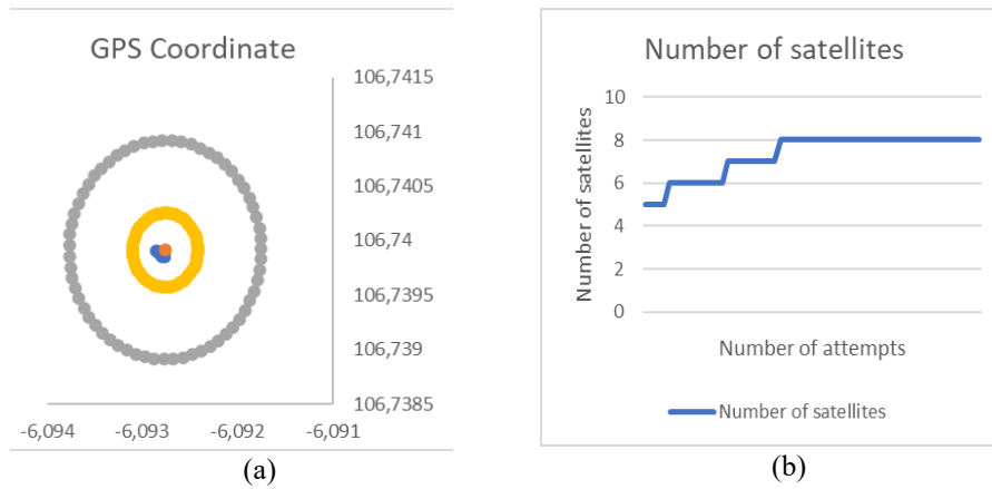
Fig. 4. Outdoor GPS Accuracy Test
