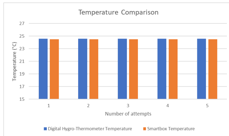
Fig. 5. Temperature Comparison Test
